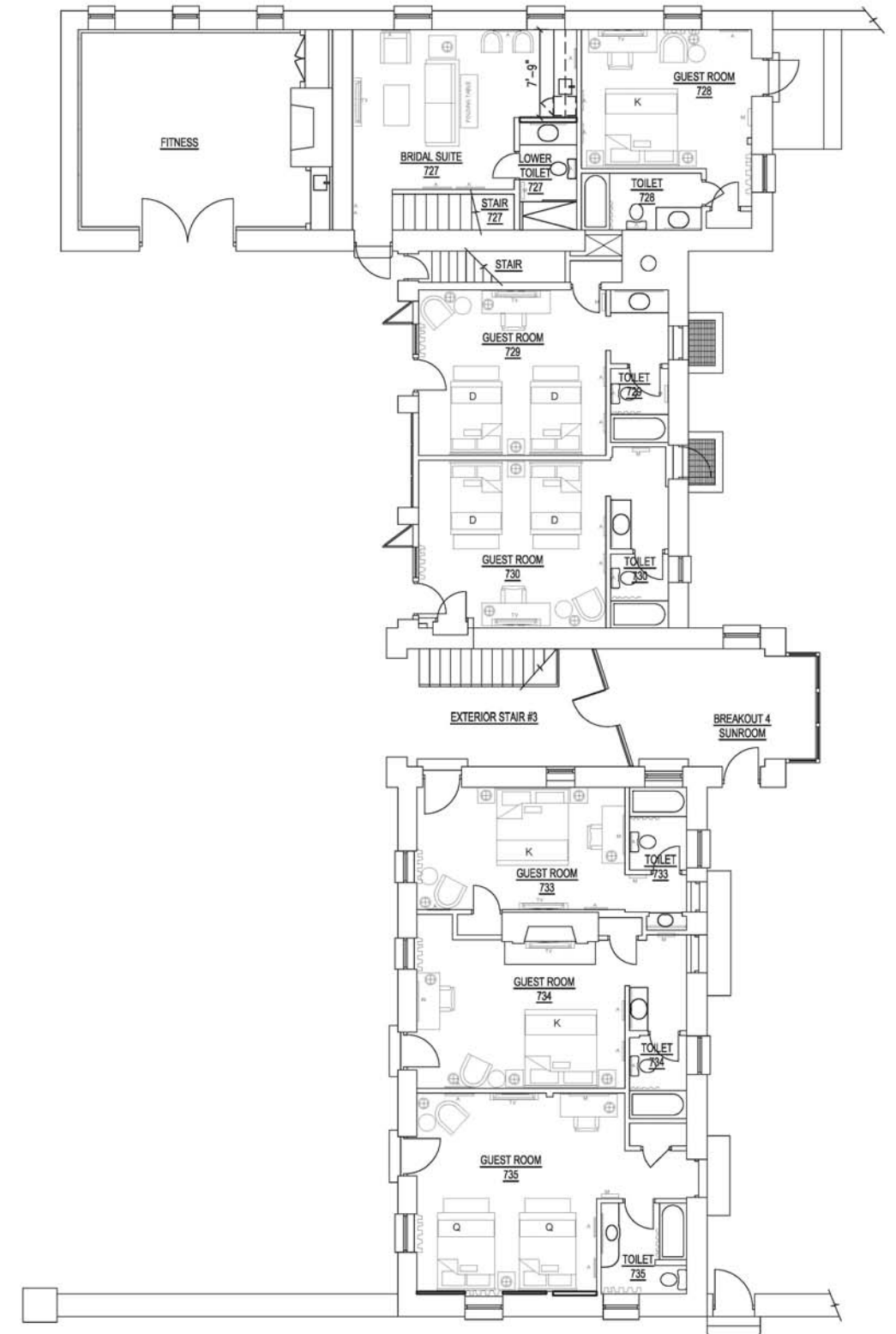
1 BUILDING A - FIRST FLOOR PLAN A1.1
