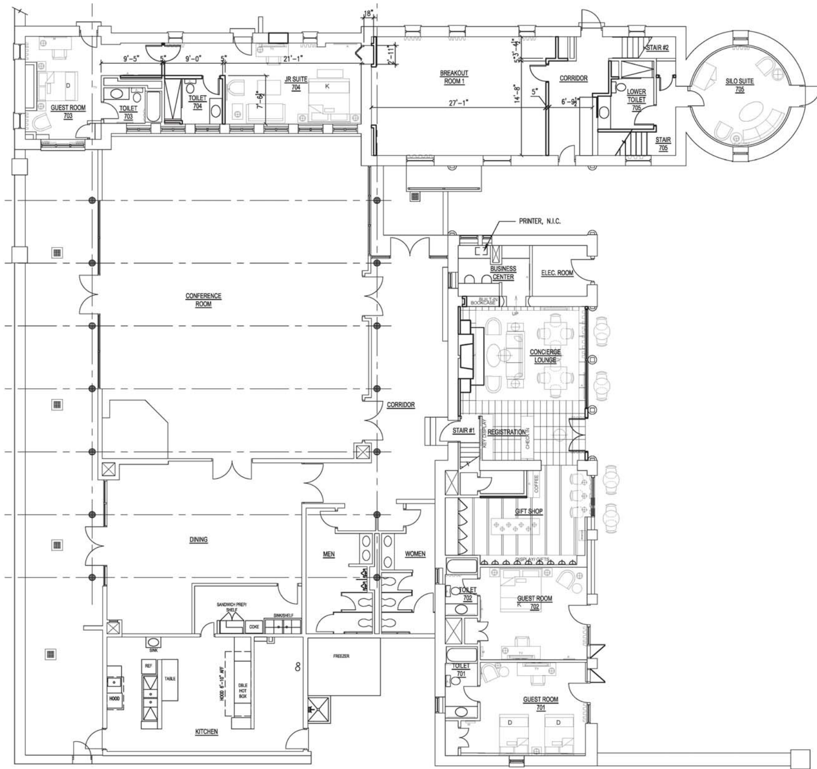
2 BUILDING B - FIRST FLOOR PLAN A1.1
